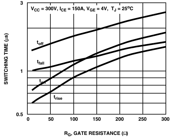
Figure 14. Switching Time vs Gate Resistance
